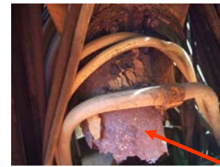
Corroded beam and saddles
